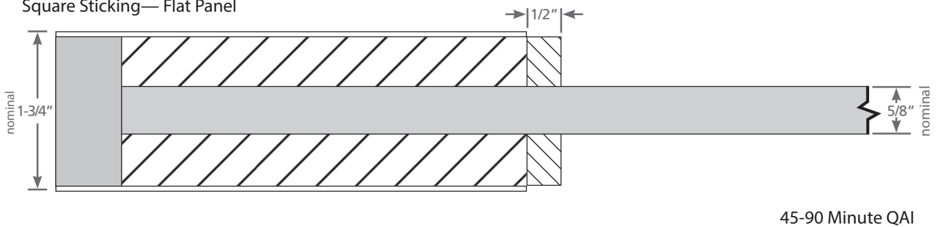
Square Sticking — Flat Panel
