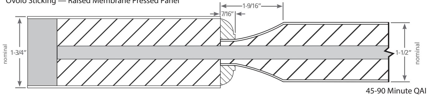
Ovolo Sticking — Raised Membrane Pressed Panel
