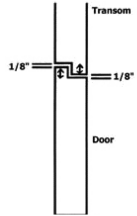
Rabbeted Transom
