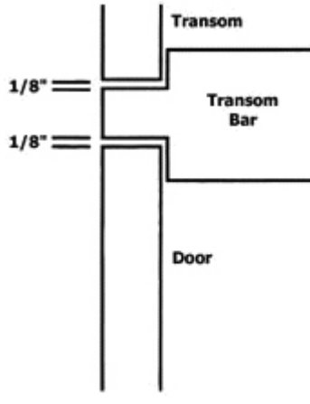
Square Transom with Fixed Bar
