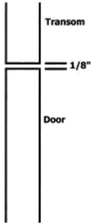
Square Transom
